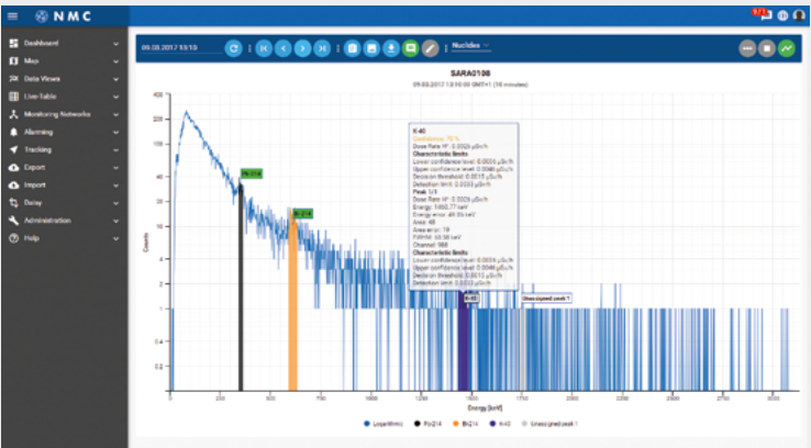
Gamma spectra display and analysis, e.g. to determine the precise causes in cases of suspected radionuclides.
